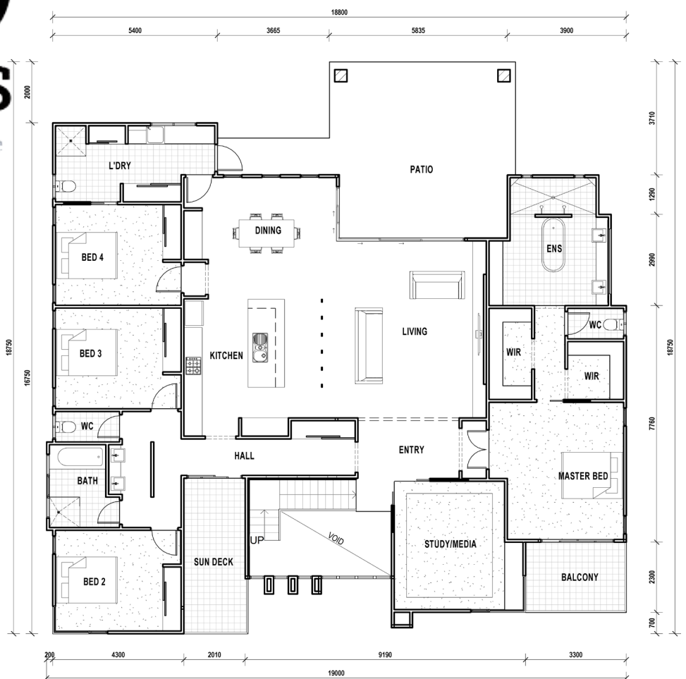
First Floor
