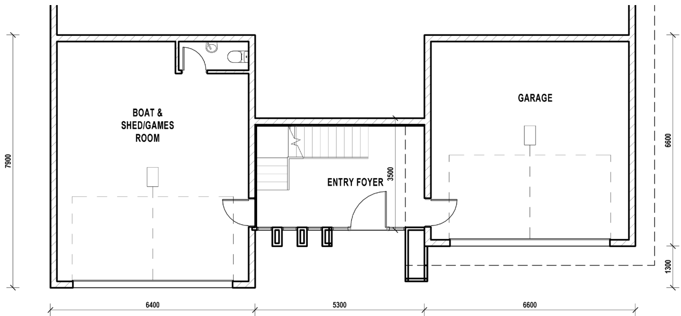
Ground Floor
